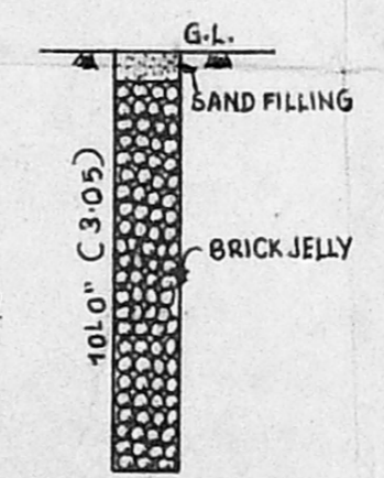
PERCOLATION PIT
